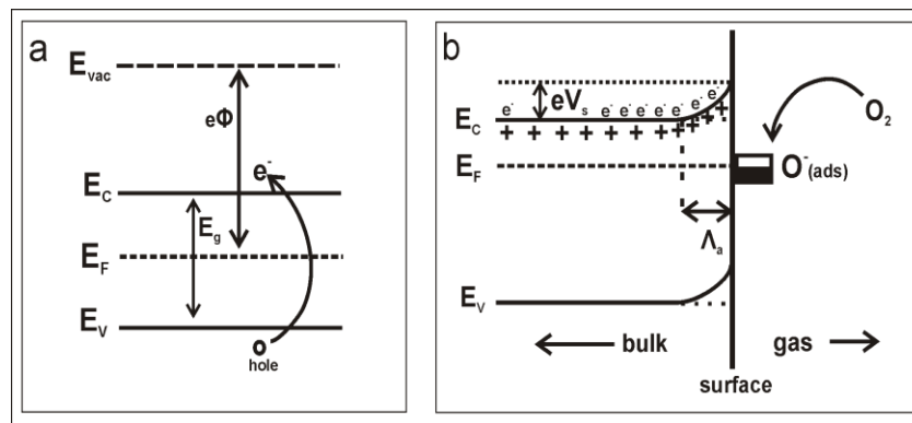
Figure 2.16: a) Simple schematic of the band diagram of a semiconductor. E v , E F , E c , E vac , E g denote the energy of the valence band, Fermi level, conduction band, vacuum level and band gap and Φ represents the work function. At 0 K, the conduction band is completely empty and at higher temperatures, electrons can jump to the conduction band leaving holes in the valence band. b) A simplified model of band bending at the surface of an n-type semiconductor after chemisorption of charged species is illustrated. Λ a denotes the thickness of the space charge layer and eV s denotes the potential barrier formed in the space charge region. The Fermi energy has the same value everywhere in the material. As a result of the surface charges accumulated on the surface due to gas adsorption, the bands bend close to the surface to keep the Fermi energy constant [188].
