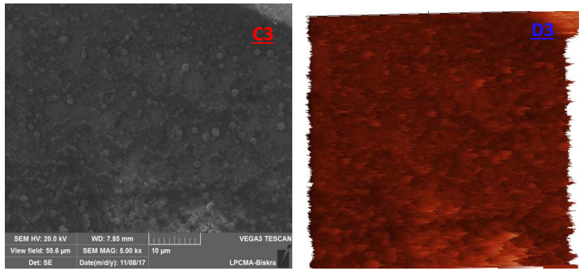
Figure 3.43: SEM and Gwyddion program images of Cu-doped NiO thin film with 6 at.% at different scales.
