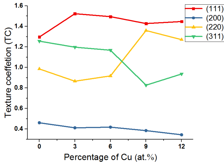
Figure 3.38: Texture coefficient values for all peaks of Cu-doped NiO thin films at different copper percentages.
