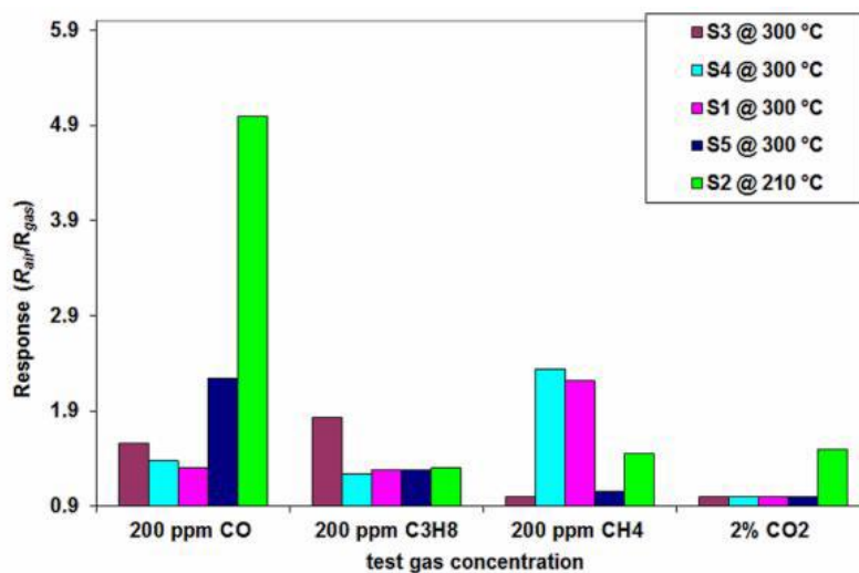
Figure 2.6: Sensors response for different gases, at the corresponding operating temperatures [182].
