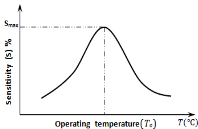
Figure 2.4: Sensitivity variation as a function of temperature at a specific concentration of gas, for the determination of operating Temperature and S_{\max} values.
