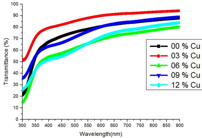
Figure 3.44: Transmission spectra of Cu-doped NiO thin films at different copper percentages.
