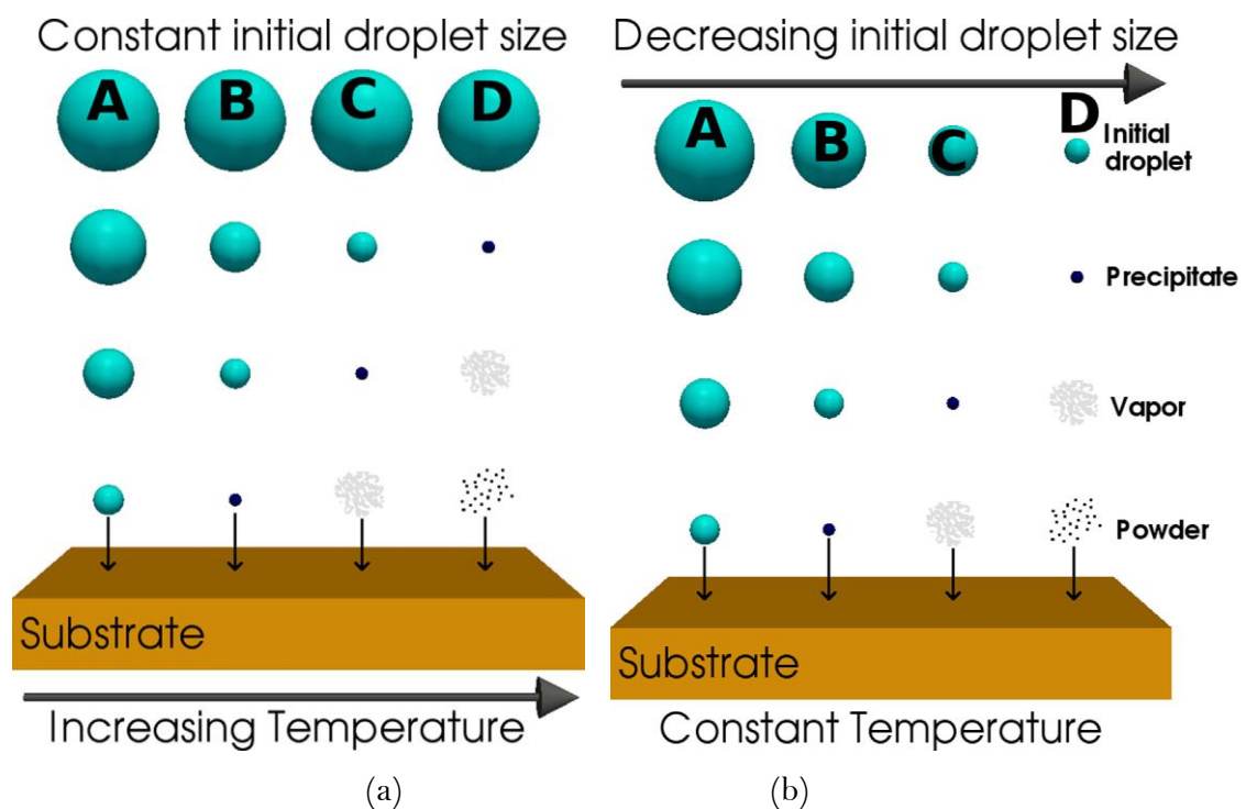
Figure 1.4: Diagram of the different process stages for the aerosol droplet evolution as it approaches the hot substrate for two cases: (a) Constant initial droplet size and increasing substrate temperature, and (b) constant substrate temperature and decreasing initial droplet size [89-90].
