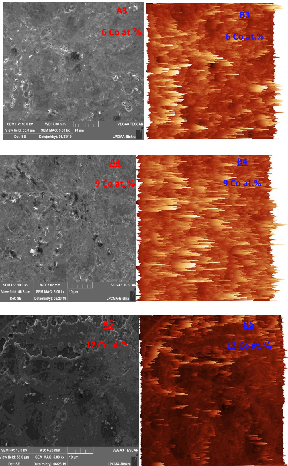
Figure 3.28: SEM and Gwyddion program images of Co-doped NiO thin films different cobalt percentages.
