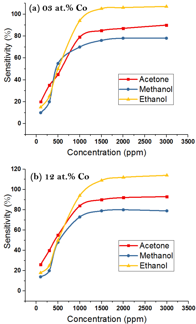
Figure 4.10: Variation of the sensitivity of the Co-doped NiO based sensors as function of concentration of methanol, ethanol and acetone vapors.
