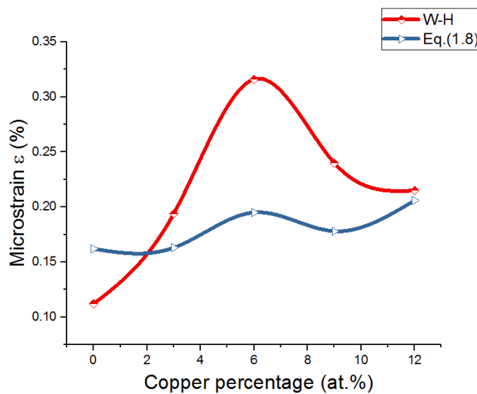
Figure 3.41: Comparison between the values of the Microstrain ( \epsilon_\mu ) determined by Williamson-Hall plot method and Eq. (1.8).
