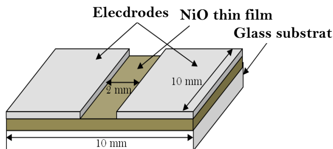
Figure 4.2: Schematic diagram of sensing element with two silver strips used as electrodes.
