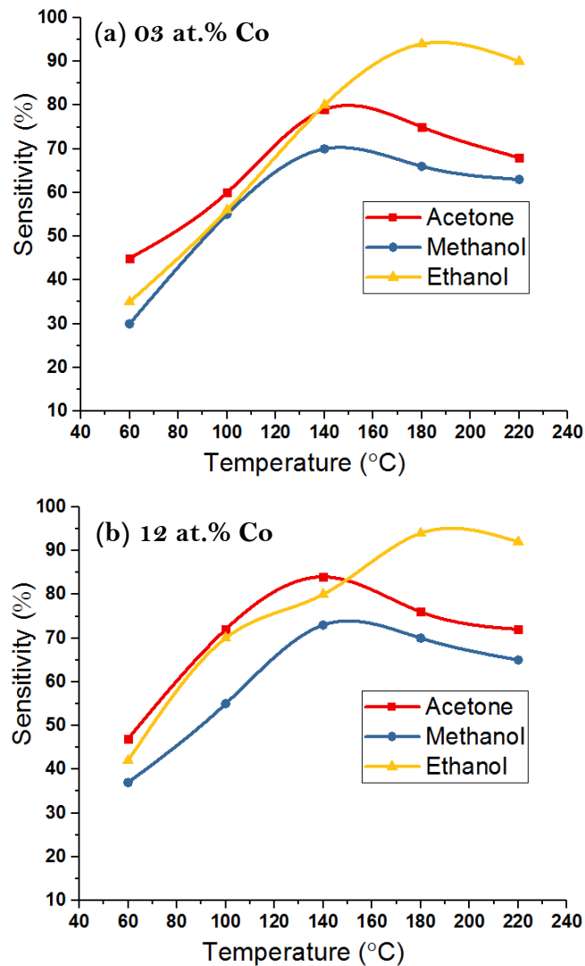
Figure 4.8: Response curves of Co-doped NiO based sensors towards methanol, ethanol and acetone (1000 ppm) at different operating temperatures.
