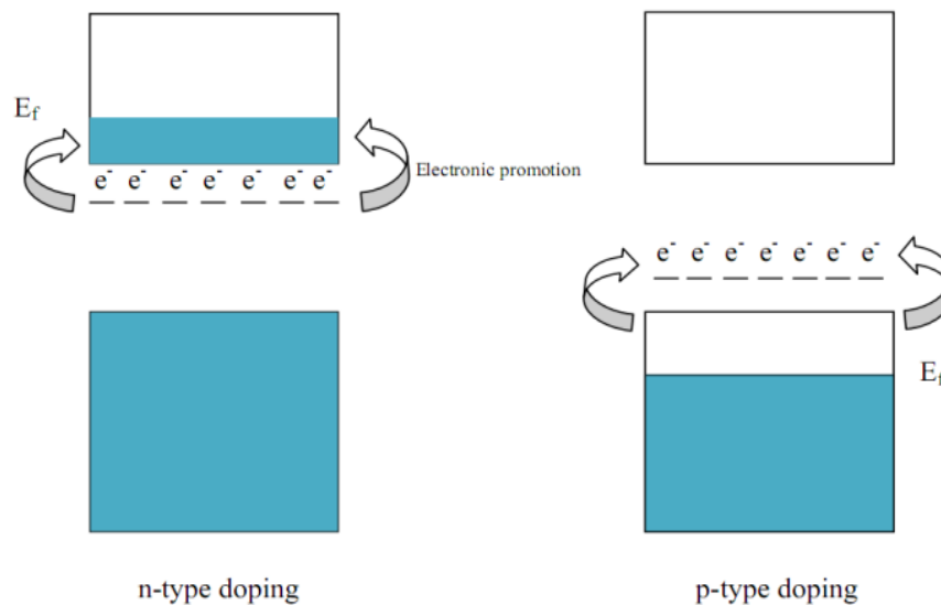
Figure 1.24: Band structure diagrams of n-type and p-type doped semiconductor materials: showing promotion of the electrons over a small defect ionisation energy level.
