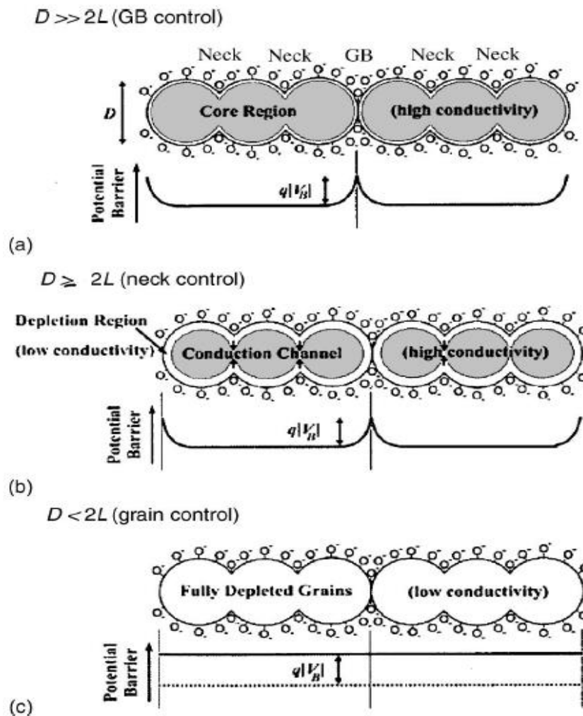
Figure 2.19: Schematic model of the effect of the crystallite size on the sensitivity of metal-oxide gas sensors: (a) D \gg 2L (GB control); (b) D \geq 2L (neck control); (c) D < 2L (grain control) [196].
