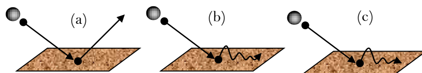
Figure 2.11: The phenomenon of: (a) scattering, (b) trapping and (c) sticking.
