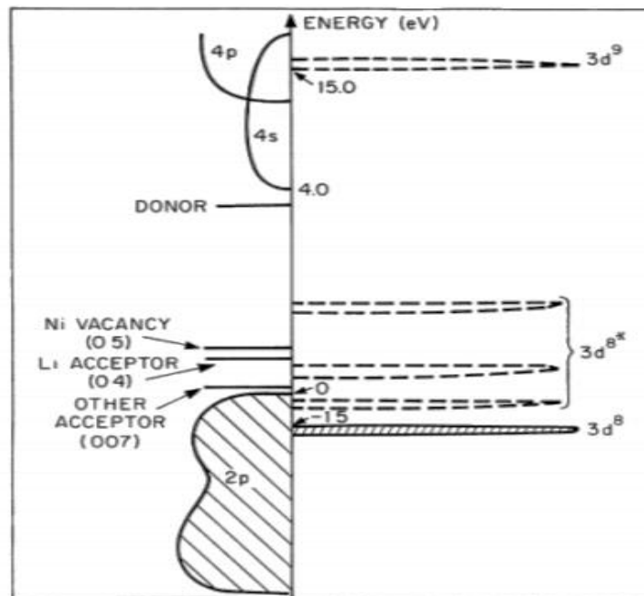
Figure 1.23: Energy diagram of density of states (pseudoparticle) in NiO.
