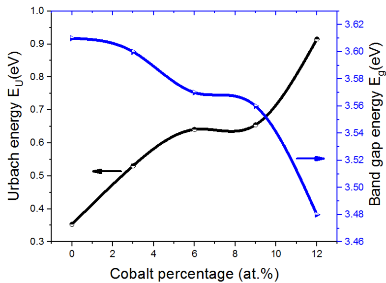
Figure 3.33: Reverse correlation between optical band gap energy and Urbach energy of Co-doped NiO thin films at different cobalt percentages.
