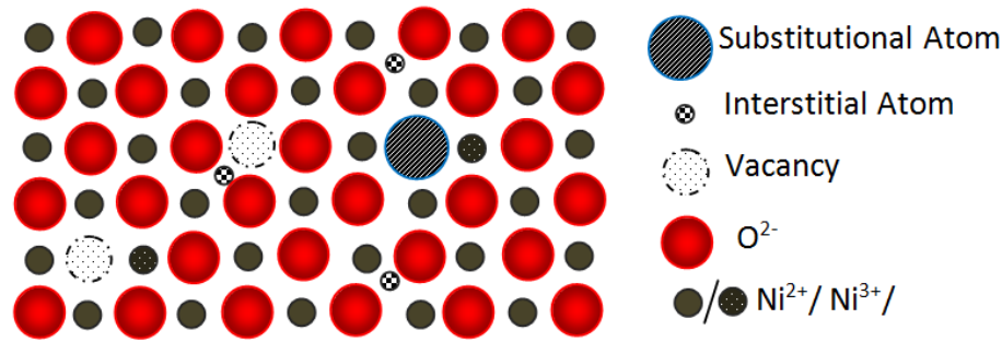
Figure 1.20: Types of point defects inside of NiO crystal.
