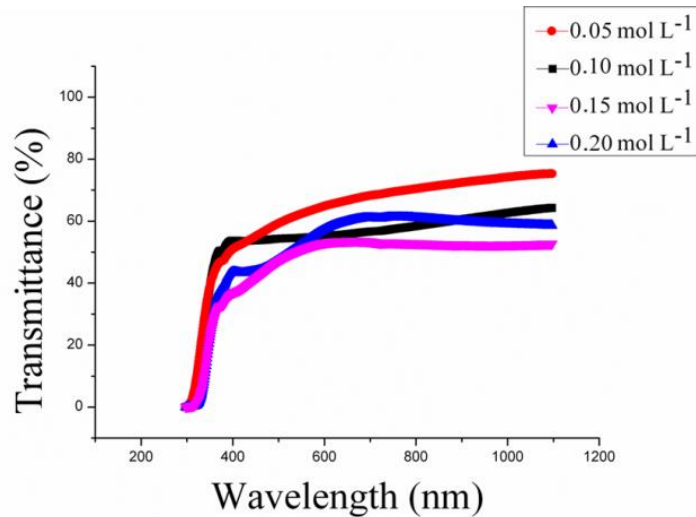
Figure 3.9: Transmission spectra of NiO samples for different precursor molarity.
