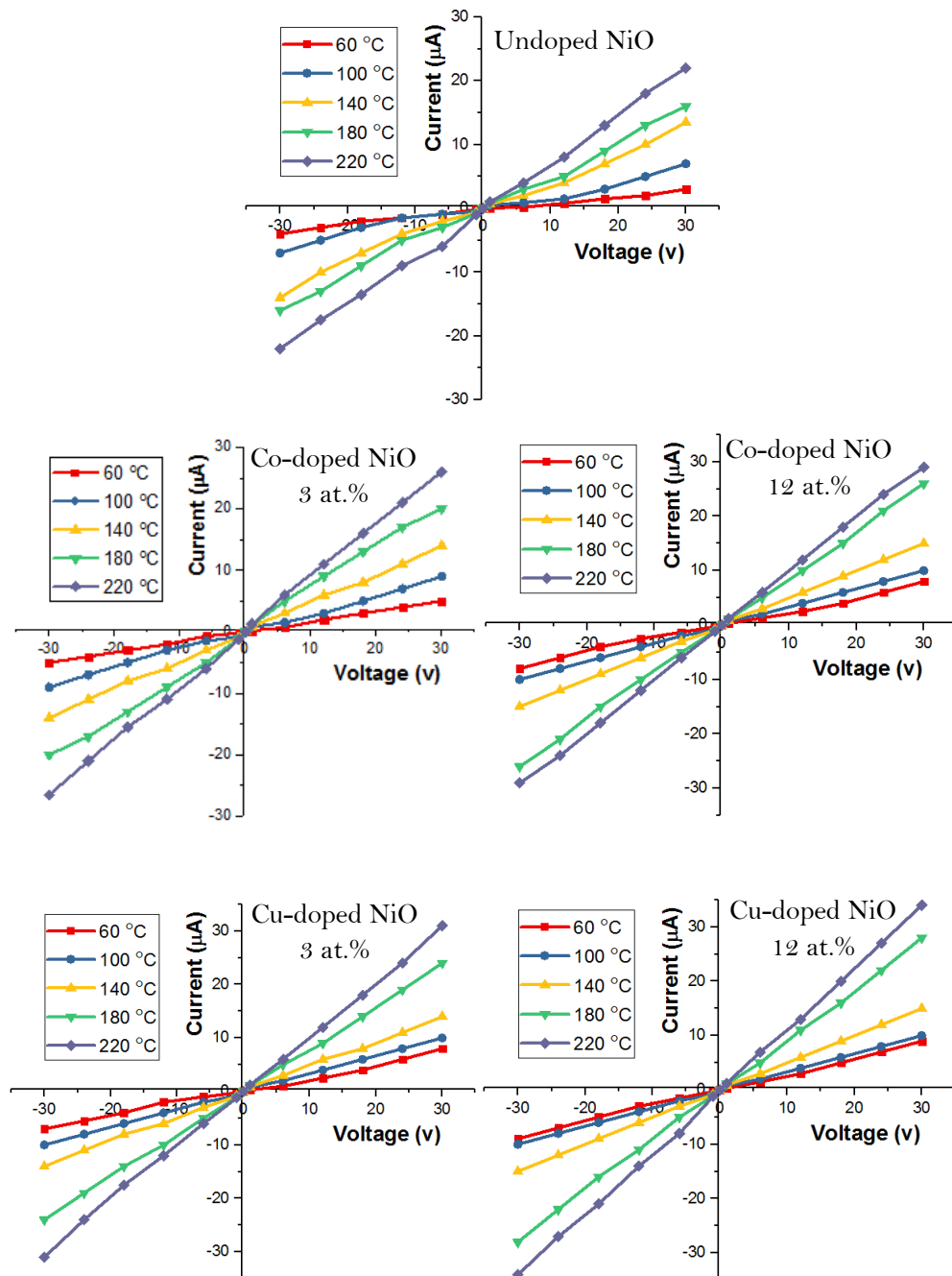
Figure 4.3: Voltage-current Plot (in air) of undoped and Co and Cu-doped NiO thin films at different operating temperature.
