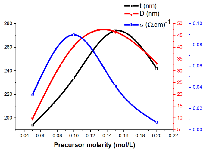
Figure 3.14: The variation of the crystallite size, the thickness and the electrical conductivity of NiO thin films as a function of the precursor molarity.
