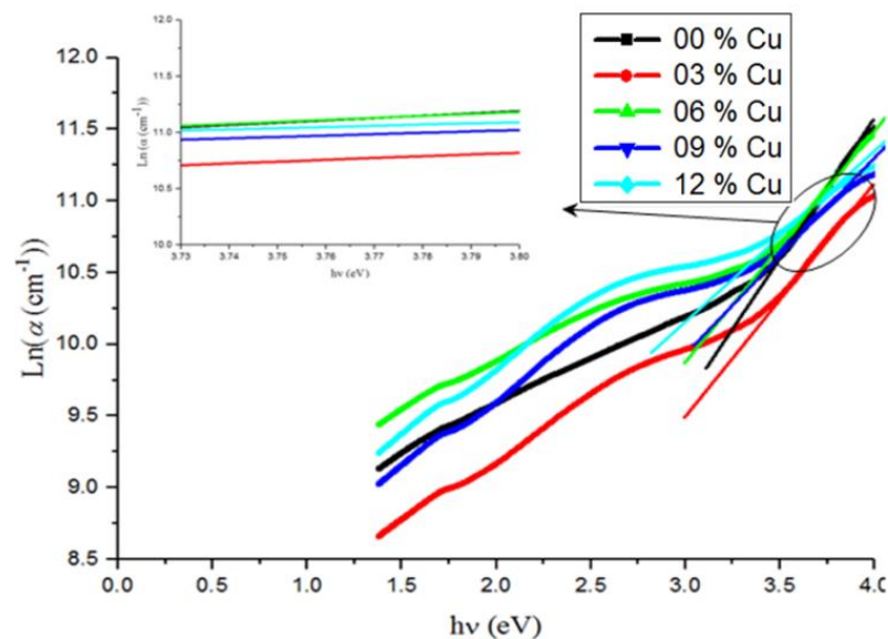
Figure 3.47: Plot of \text{Ln}(\alpha) versus incident photon energy ( h\nu ) of Cu-doped NiO thin films at different copper percentages.
