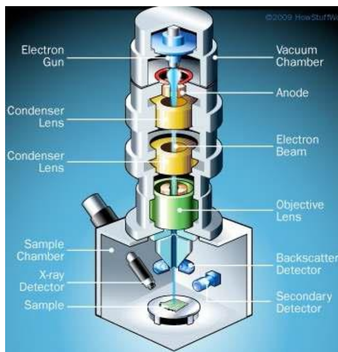
Figure 1.10: Schematic representation of scanning electron microscope [119].
