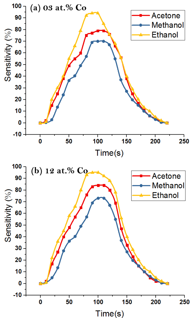
Figure 4.9: Response of Co-doped NiO based sensors towards 1000 ppm of ethanol, acetone and methanol at the optimum operating temperatures.
