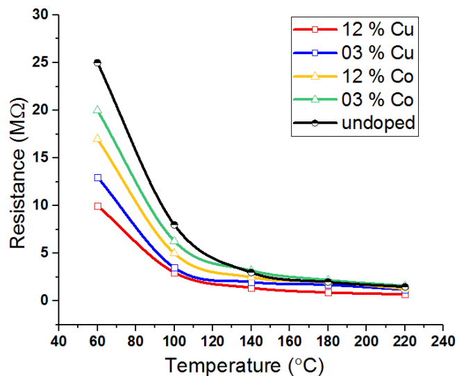
Figure 4.16: Variation of resistance (in air) of undoped and Co and Cu-doped NiO based sensors at different operating temperatures.
