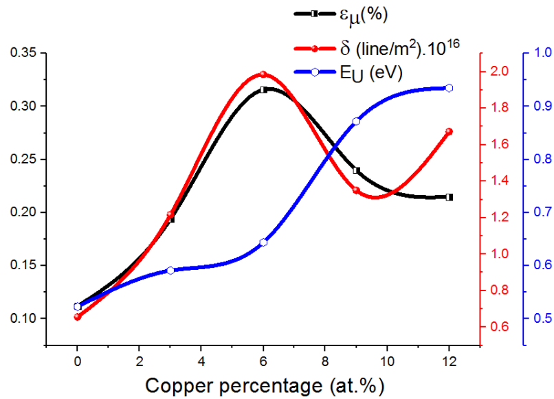
Figure 3.48: Variation of microstrain, dislocation density and Urbach energy of Cu-doped NiO thin films at different copper percentages.
