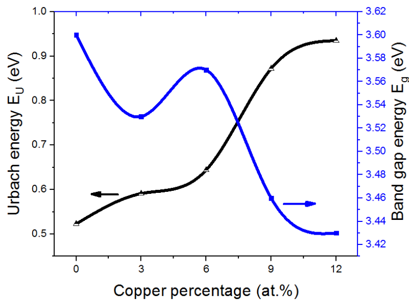
Figure 3.49: Variation of optical band gap energy and Urbach energy of Cu-doped NiO thin films at different copper percentages.
