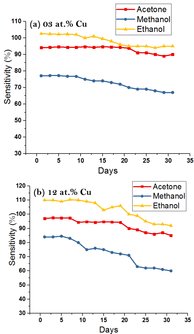
Figure 4.15: Stability characteristics of Cu-doped NiO based sensors.
