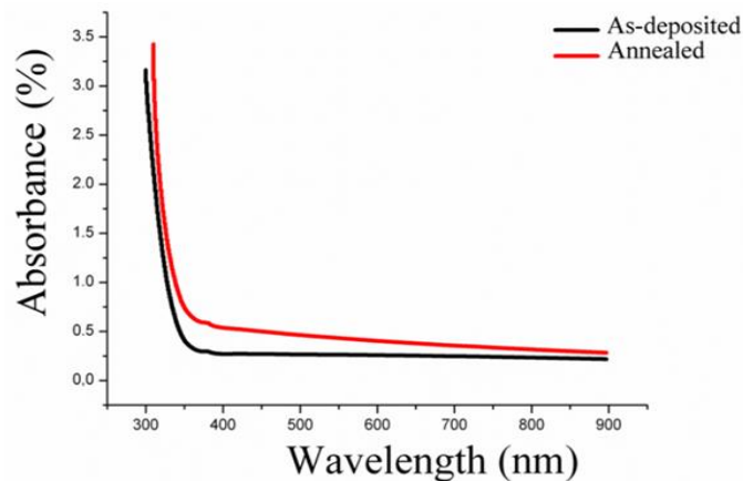
Figure 3.17: Absorbance spectra of the as-deposited and annealed NiO thin films.
