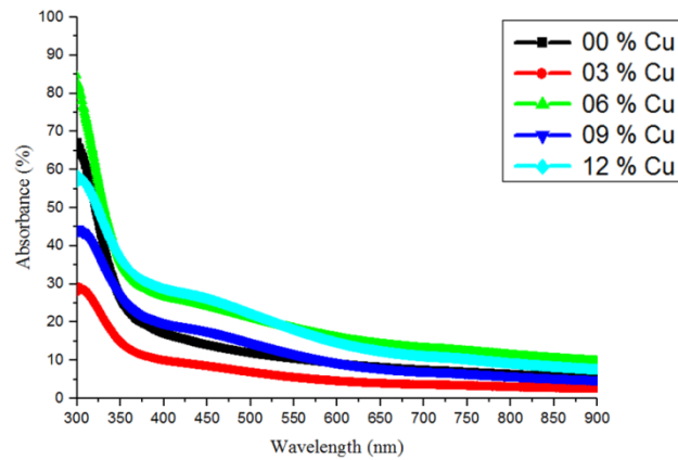
Figure 3.45: Absorbance spectra of Cu-doped NiO thin films at different copper percentages.
