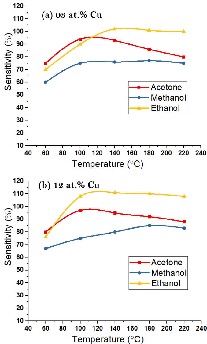
Figure 4.12: Response curves of Cu-doped NiO based sensor towards methanol, ethanol and acetone (1000 ppm) at different operating temperatures.
