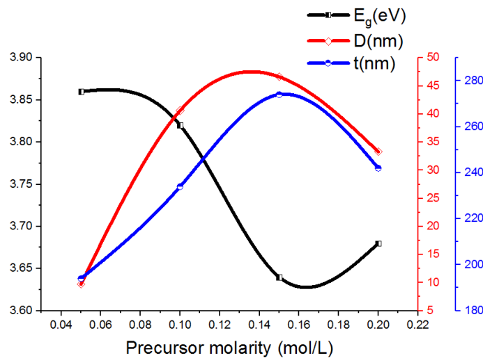
Figure 3.13: The correlation between the crystallite size and thickness with band gap energy of NiO thin films as a function of the precursor molarity.
