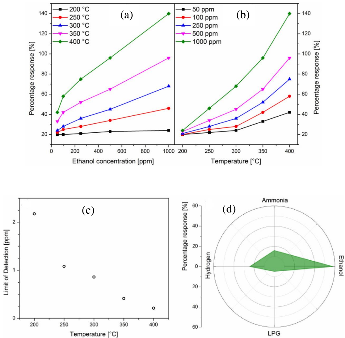
Figure 2.10: Percentage response as a function of (a) ethanol concentration and (b) working temperature, (c) limit of detection as a function of the sensor operating temperature (Polycrystalline NiO nanowires) and (d) selectivity plot at 200 °C for 100 ppm of gas [186].
