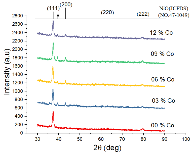
Figure 3.23: XRD patterns of the deposited Co-doped NiO thin films on glass substrate at different cobalt percentages.
