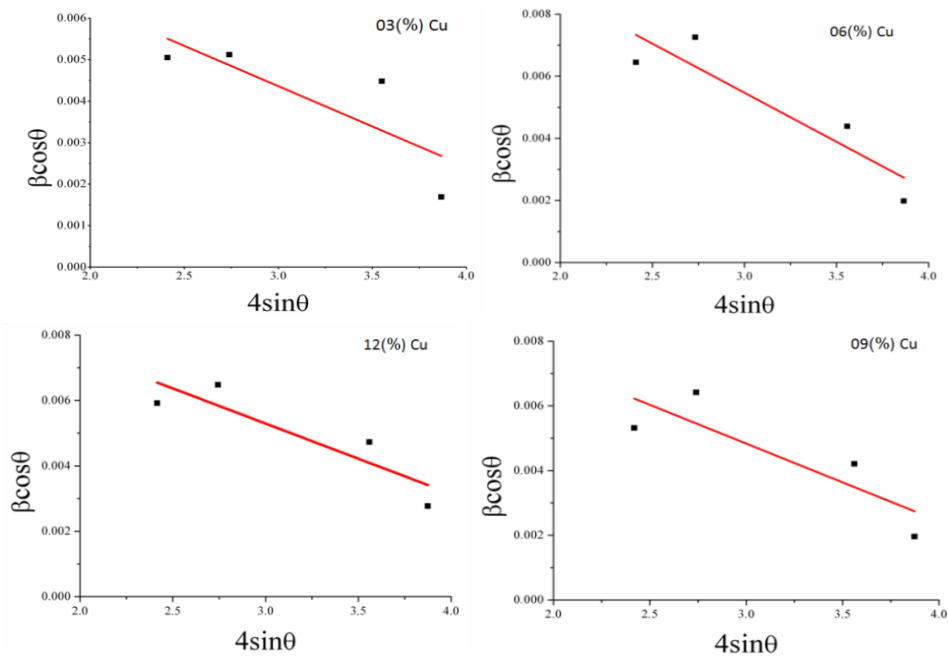
Figure 3.39: Determination of the average crystallite size ( D ) and the microstrain ( \varepsilon_{\mu} ) by Williamson-Hall plot method.
