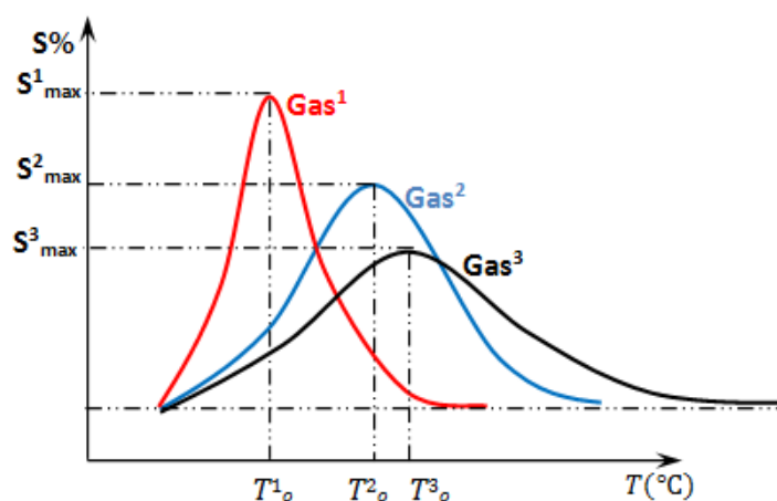
Figure 2.7: Variation of the values and forms of response as a function of the temperature variation for different gases having the same concentration.
