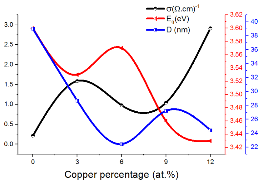
Figure 3.50: Variation of electrical conductivity, optical band gap energy and crystallite size of Cu-doped NiO thin films at different copper percentages.
