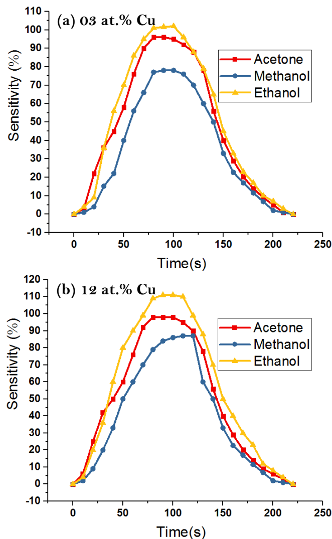
Figure 4.13: Responses of Cu-doped NiO based sensors towards 1000 ppm of ethanol, acetone and methanol at the optimum operating temperatures.
