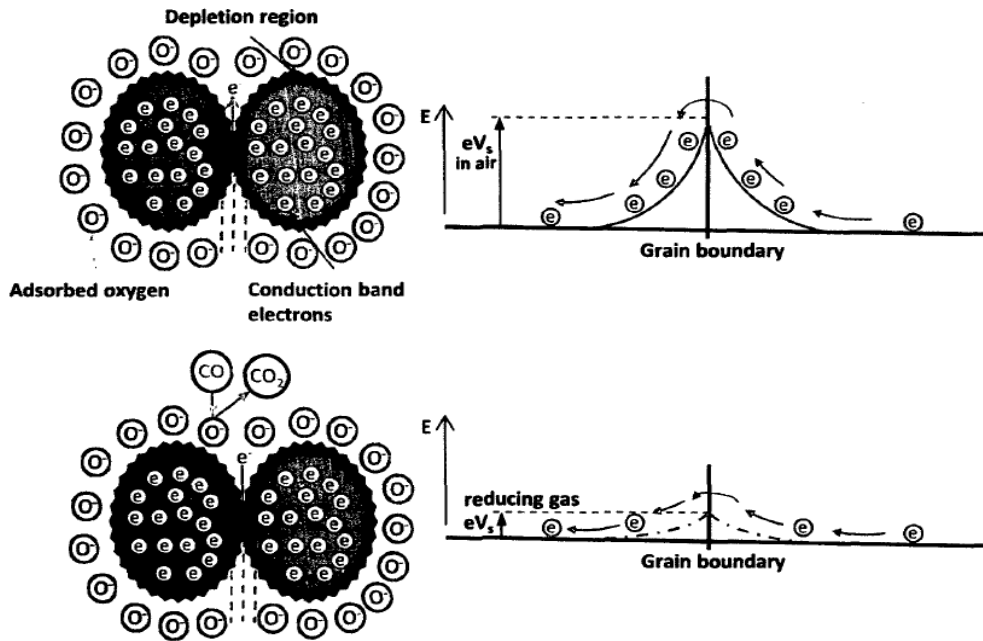
Figure 2.14: Gas sensing mechanism of metal oxide semiconductor [190].
