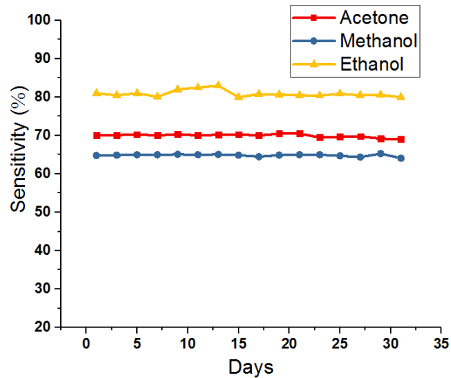
Figure 4.7: Stability characteristics of undoped NiO based sensor.
