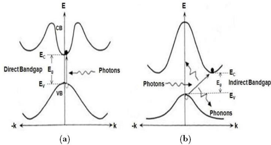
Figure 1.13: Direct (a) and indirect (b) band gap.
