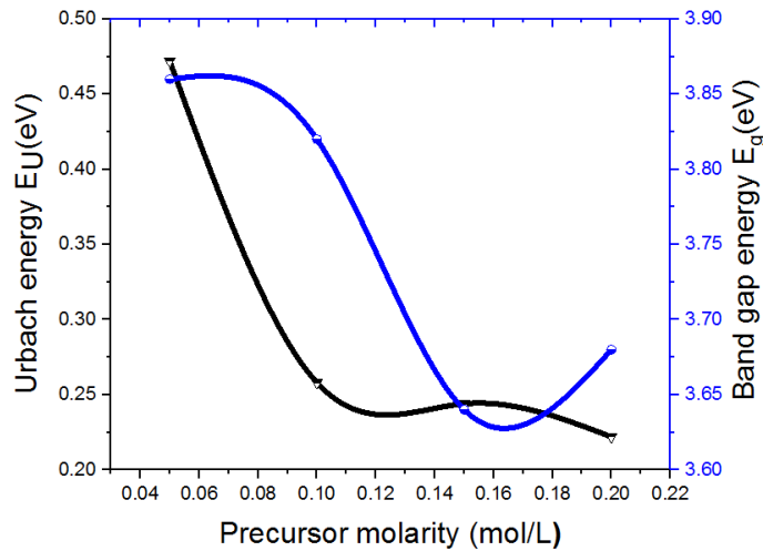
Figure 3.12: The variation Urbach energy and band gap energy of NiO thin films as a function of the precursor molarity.
