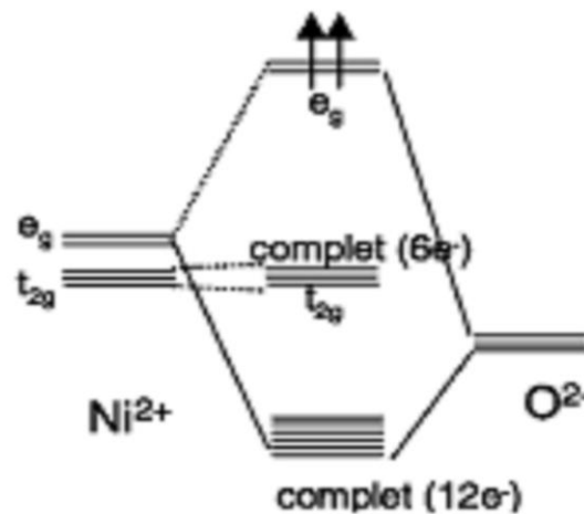
Figure 1.21: Schematic diagram of NiO energy levels.
