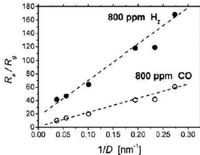
Figure 2.18: Influence of crystallite size on sensitivity ( R_a/R_g ) at 300°C [196].
