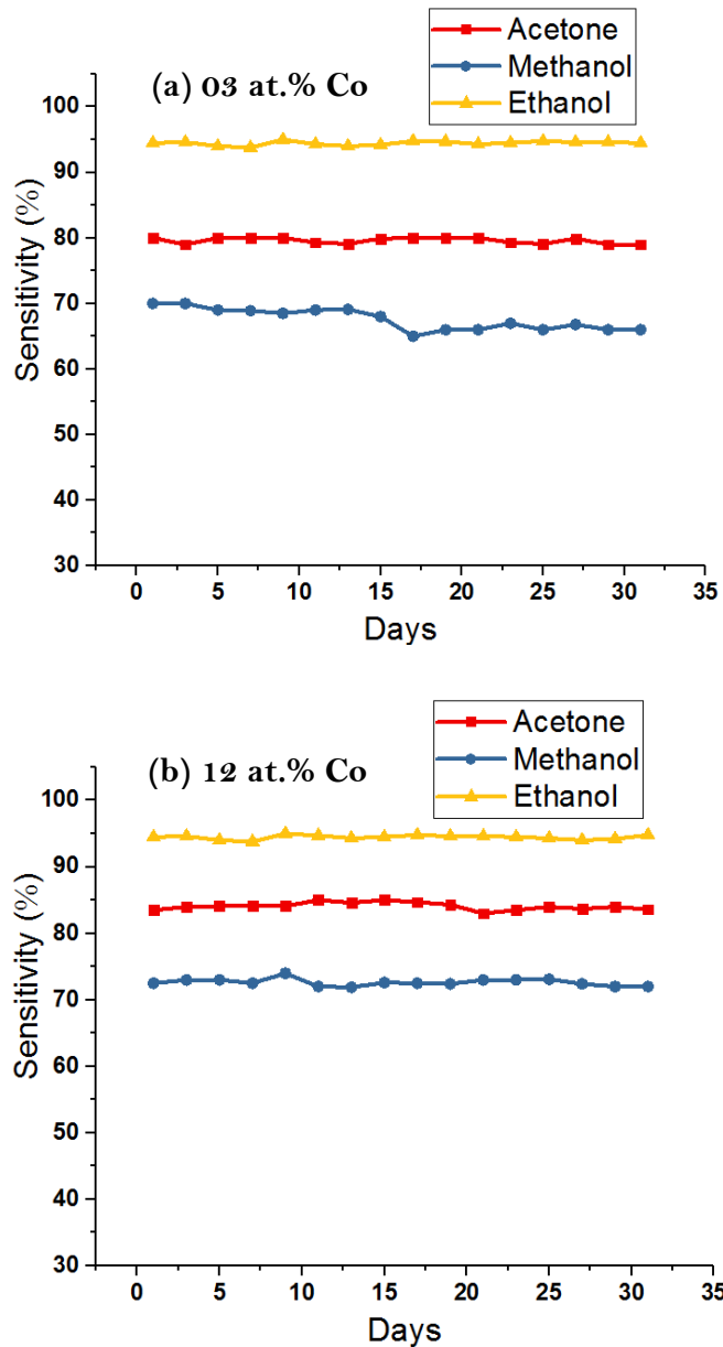
Figure 4.11: Stability characteristics of Co-doped NiO based sensors.
