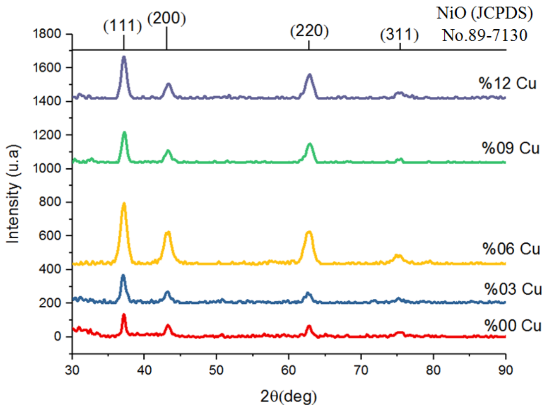
Figure 3.36: XRD patterns of the deposited Cu-doped NiO thin films on glass substrate at different copper percentages.
