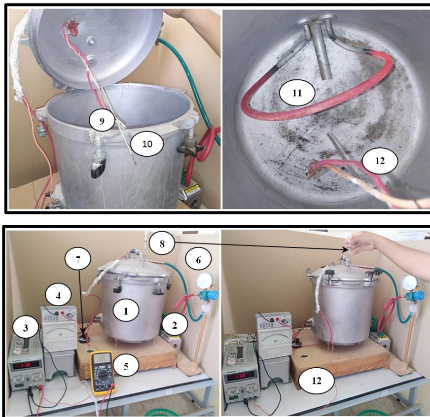
Figure 4.1: The most important components of the homemade gas sensor.
