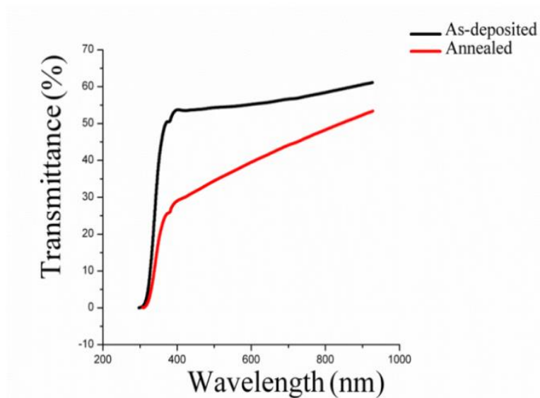
Figure 3.19: Transmission spectra of the as-deposited and annealed NiO thin films.
