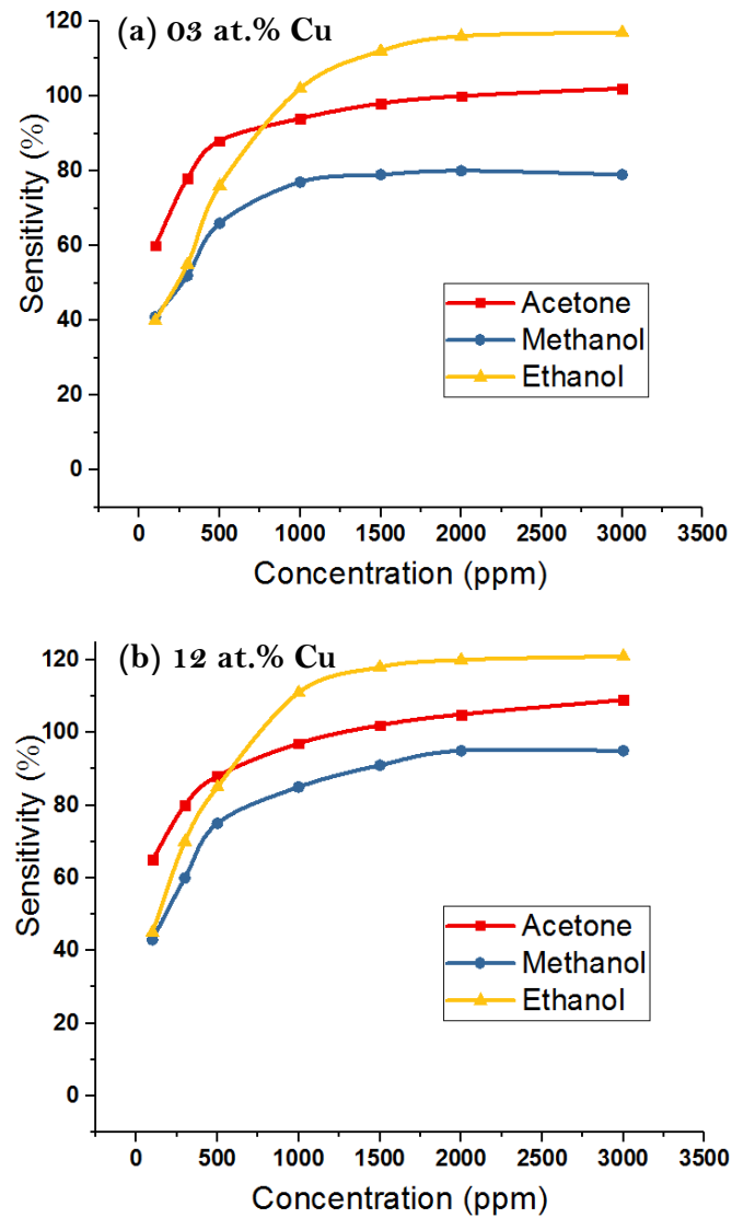
Figure 4.14: Variation of the sensitivity of Cu-doped NiO based sensors as function of concentration of vapors.
